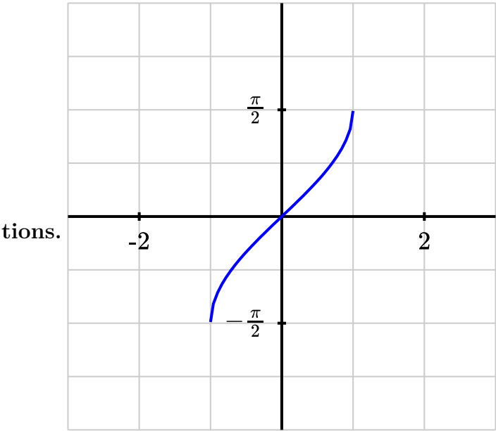
Figure A.1.21 Graph of y = \sin^{-1}(x)
