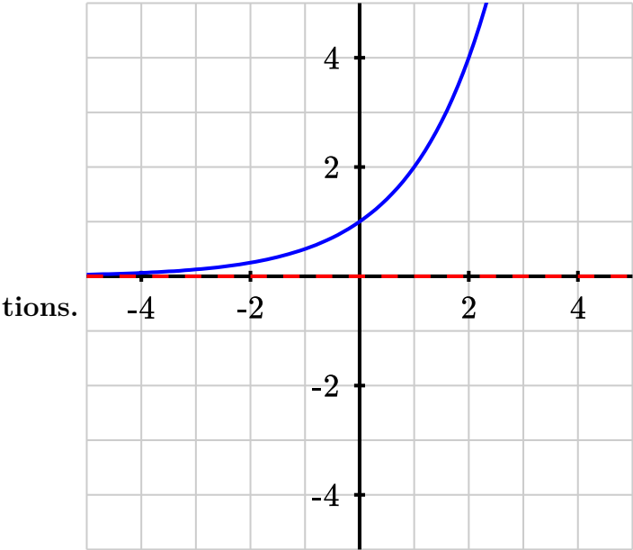
Figure A.1.11 Graph of y = b^x , with b = 2 Figure A.1.12 Graph of y = \log_b x , with b = 2
