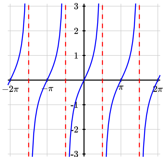
Figure 7.2.12 y = \tan(x)
