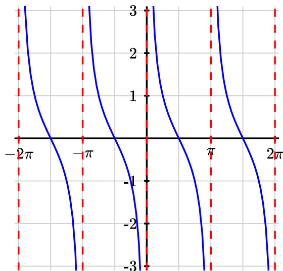
Figure 7.2.13 y = \cot(x)
