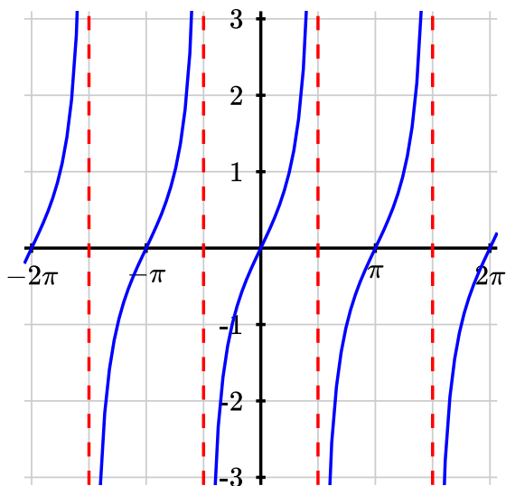
Figure 7.2.12 y = \tan(x)
