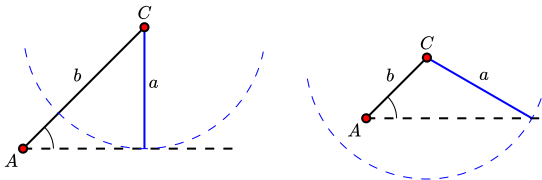
Figure 8.5.20 If the length of a is the same as the height of the triangle, the two possibilities converge and there is a single solution of a right triangle. On the other hand, if the length of a increases enough, the potential second solution swings past the angle A and thus does not exist.
